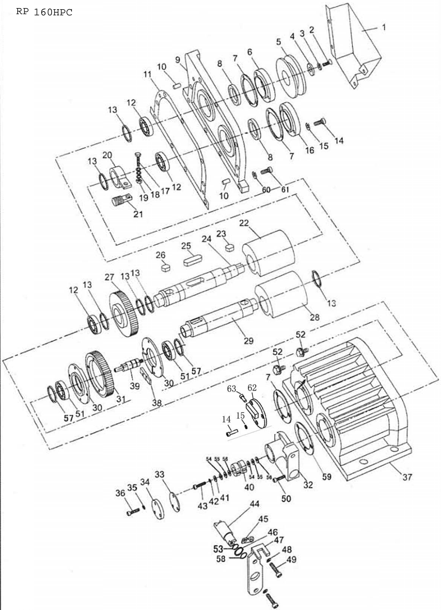
Vibrator Assembly
